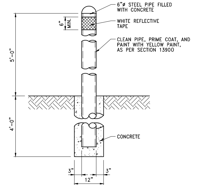
STEEL PIPE BOLLARD DETAIL NO SCALE
