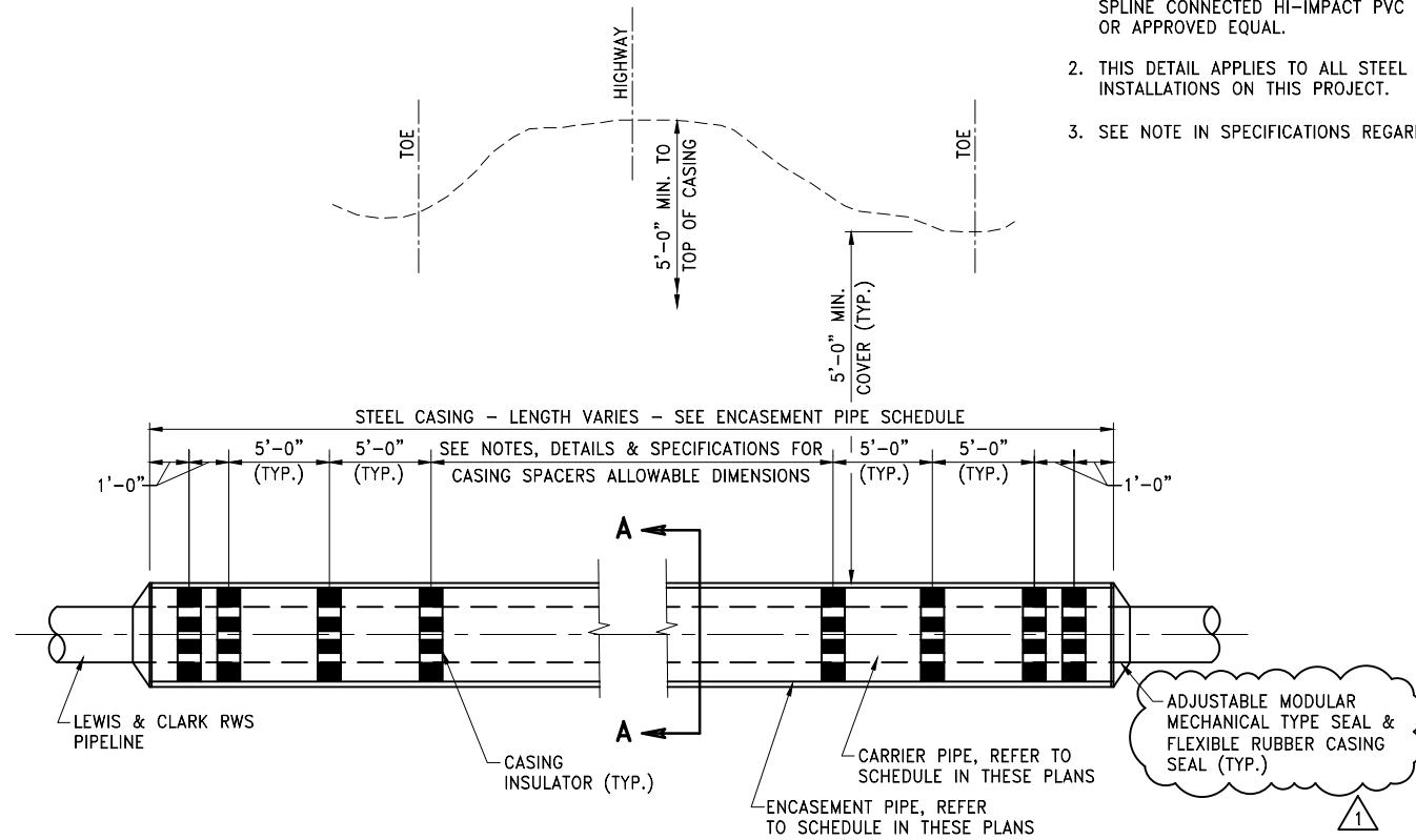
TYPICAL ENCASEMENT PIPE JACKING SECTION NO SCALE
