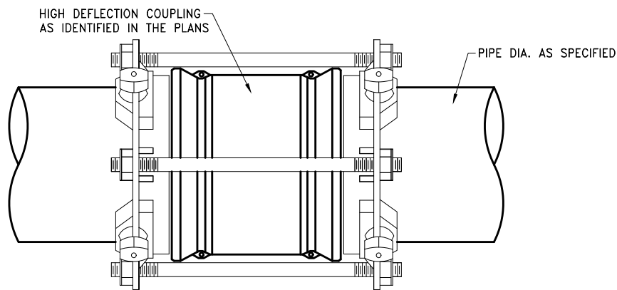
HIGH DEFLECTION COUPLING DETAIL NO SCALE
